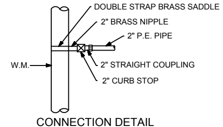
CONNECTION DETAIL
