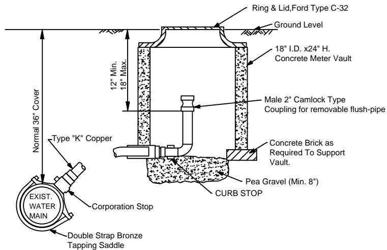
TYPICAL MANUAL AIR RELEASE VALVE INSTALLATION N.T.S.
