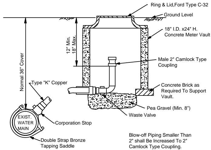
TYPICAL FLUSHING DEVICE INSTALLATION N.T.S.
