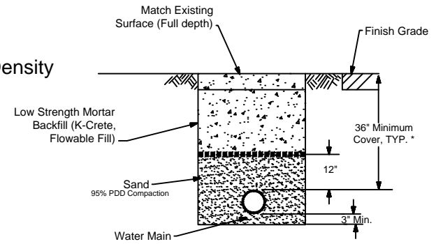
UNDER SHOULDER OF STATE MAINTAINED STREET
