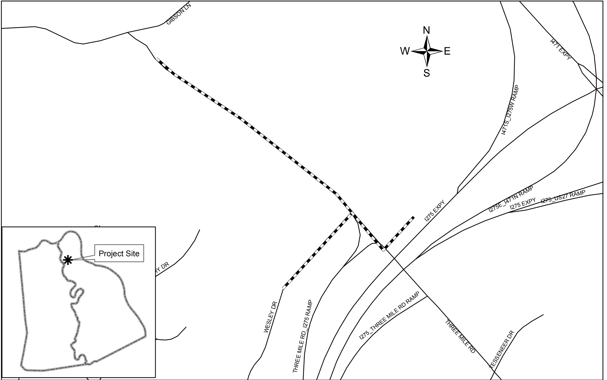
Wesley Drive and Three Mile Road water main extension
